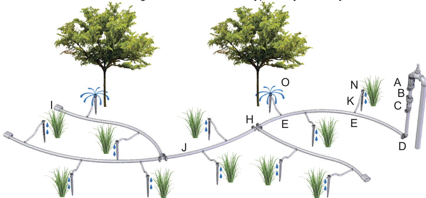
Natives and Drought Tolerant Gardens Typical System Layout
