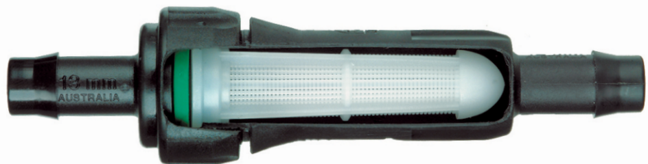
In-Line Filter cut away detail
