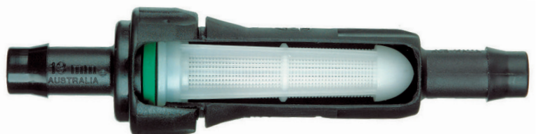
In-Line Filter cut away detail
