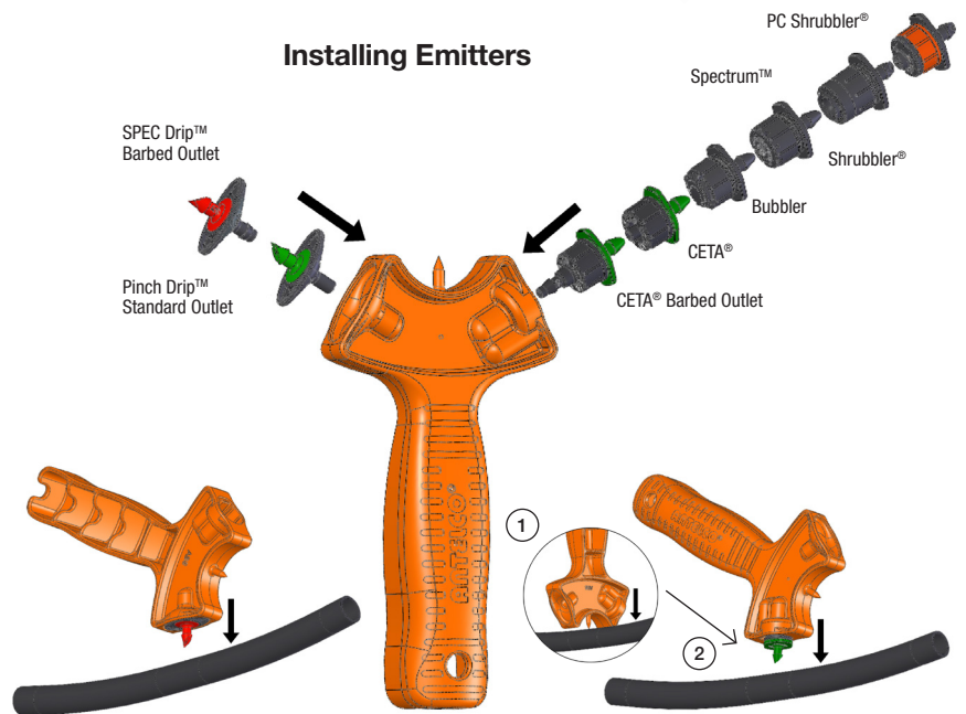
Direct insertion into lateral with the new Antelco self piercing SPEC Drip™
